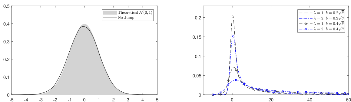
Fig. 6. Finite-sample distributions of the standardized test statistic T_{c,\epsilon} in the presence of noise. We plot the finite-sample distribution under the null (solid line) and compare it with the simulated standard normal (shaded area). Jumps are simulated with a compounded Poisson process with the intensity \lambda , and their sizes follow a double exponential distribution with location parameter 0 and scale parameter b . We consider different parameter choices: (i) \lambda = 1 , b = 0.2\sqrt{\theta} (dash), (ii) \lambda = 2 , b = 0.2\sqrt{\theta} (dash-dot), (iii) \lambda = 1 , b = 0.4\sqrt{\theta} (dash-circle), and (iv) \lambda = 2 , b = 0.4\sqrt{\theta} (dash-square). In all cases, we select the pre-averaging window k_n = \lceil \theta\sqrt{N} \rceil = 46 with \theta = 0.3 , the PDS barrier width c = 5\sigma(\bar{r}_t) , and the censoring parameter \epsilon = 0.05 .
